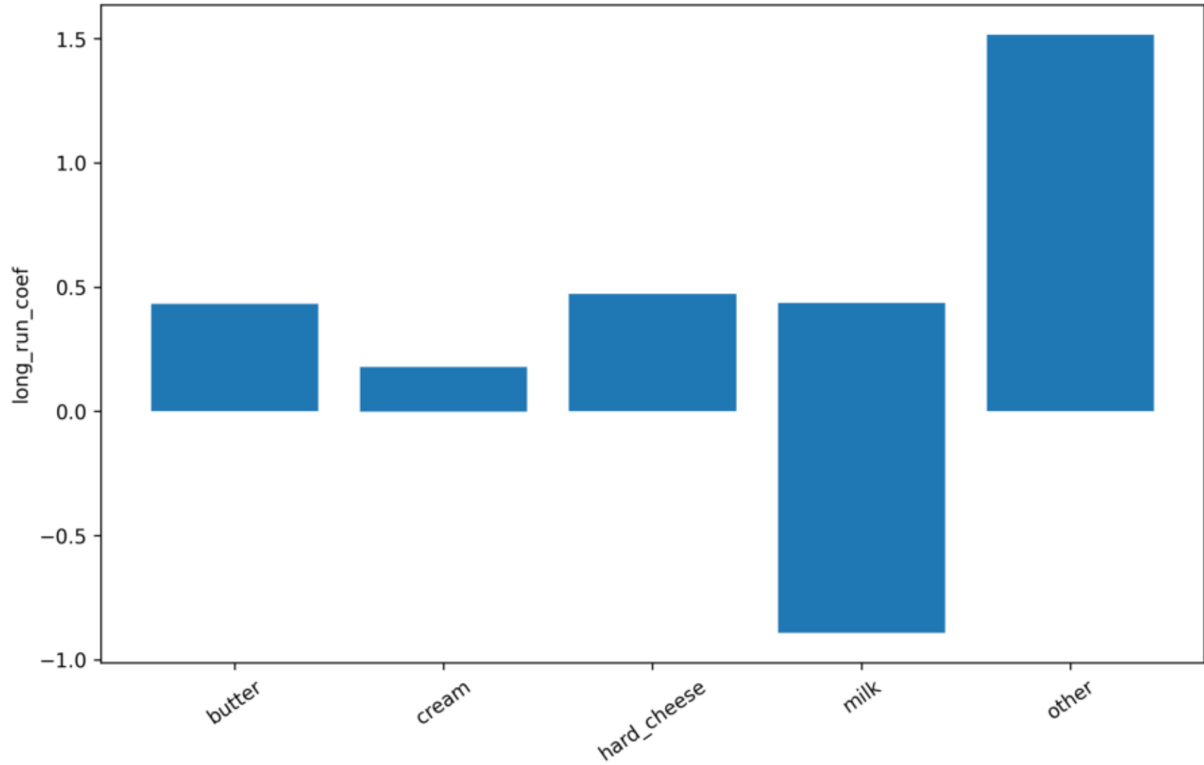
NARDL Long-run Asymmetry Proxy
