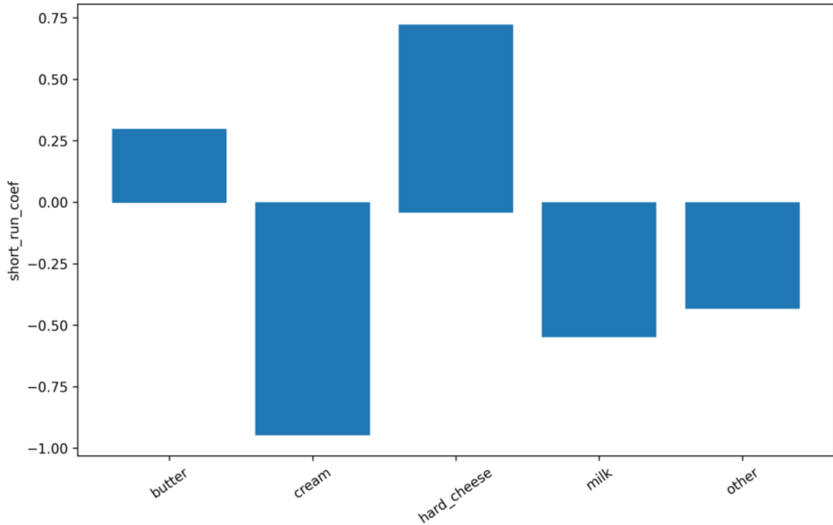
NARDL Short-run Coefficients
